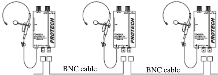
Maximum 10 sets of FD-300A can be used. BNC cables can be used up to 2km as total length.
