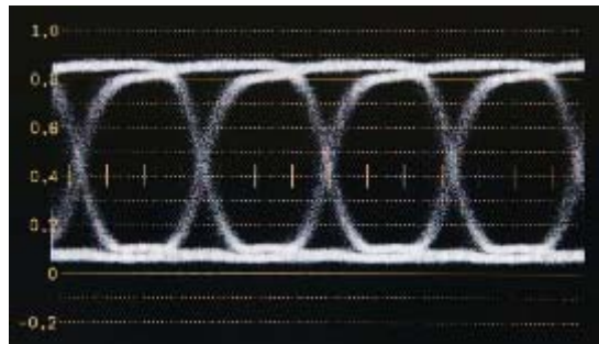
Eye Pattern
