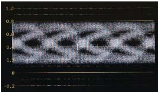
Eye Pattern
